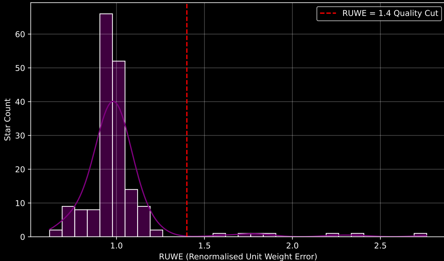
GAPOGEE DR17 Field [024-03] RUWE Distribution (n= 177)
