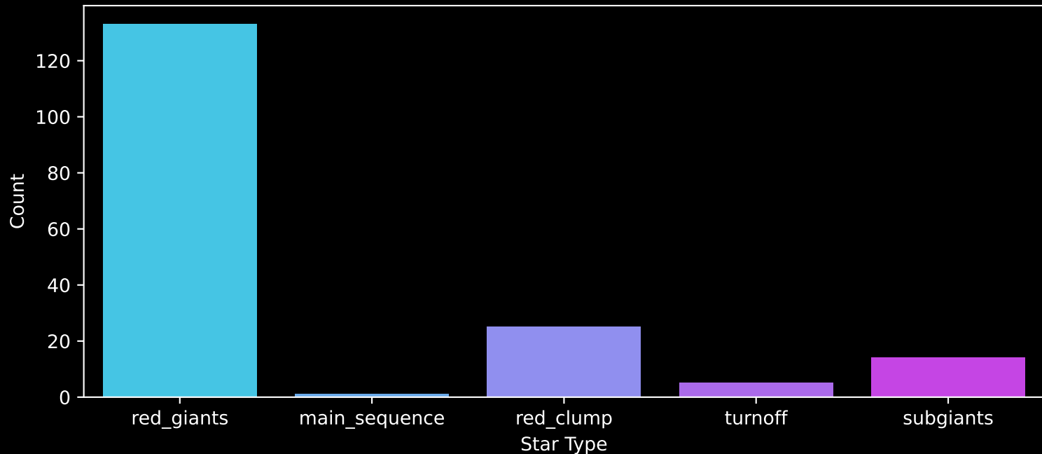
APOGEE DR17 Field: [024-03] Count plot of Star Type
