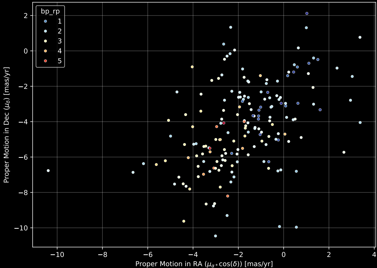
APOGEE DR17 Field: [024-03] Proper Motion Diagram (n= 178)
