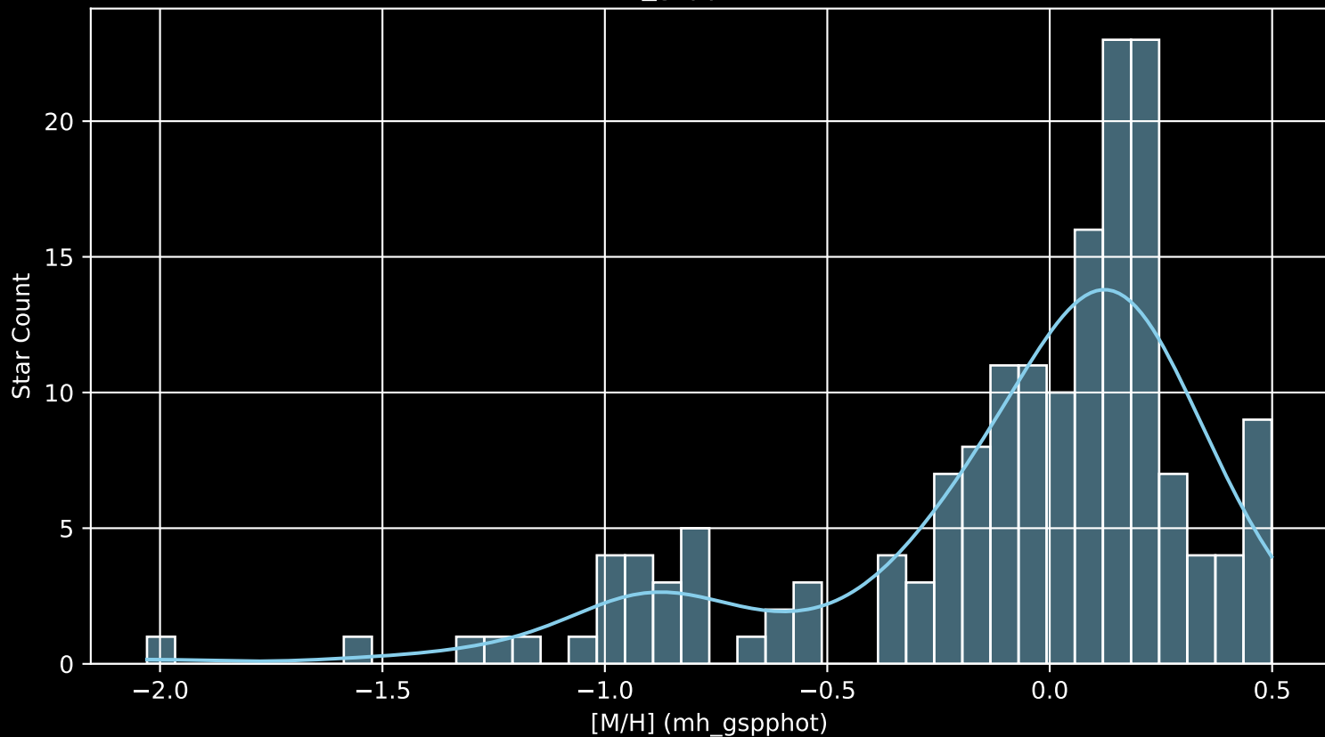
APOGEE DR17 Field: [024-03 [M/H] (mh_gspphot) (n= 168)
