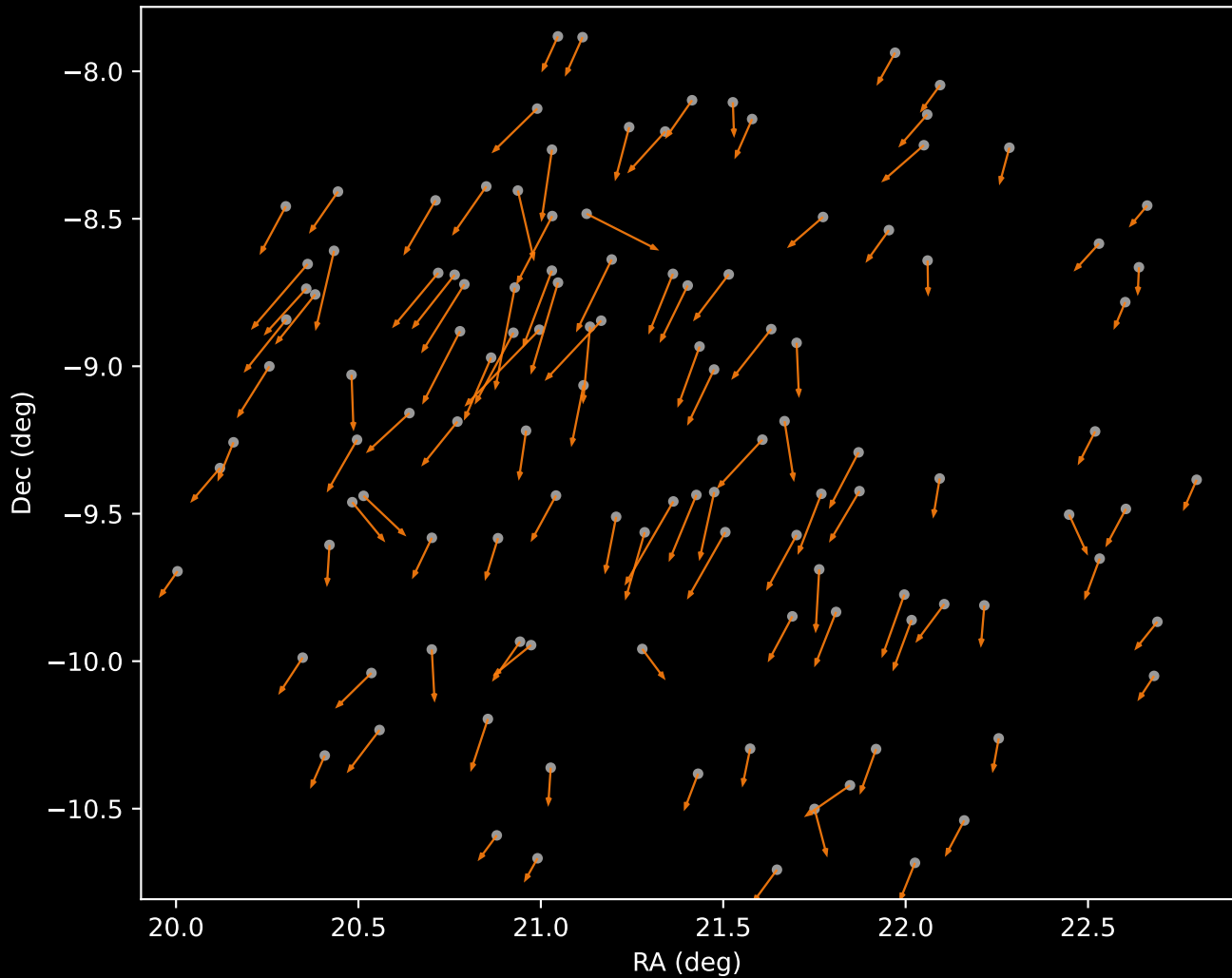
APOGEE DR17 Cluster 2 Proper Motion Vectors (n=117)
