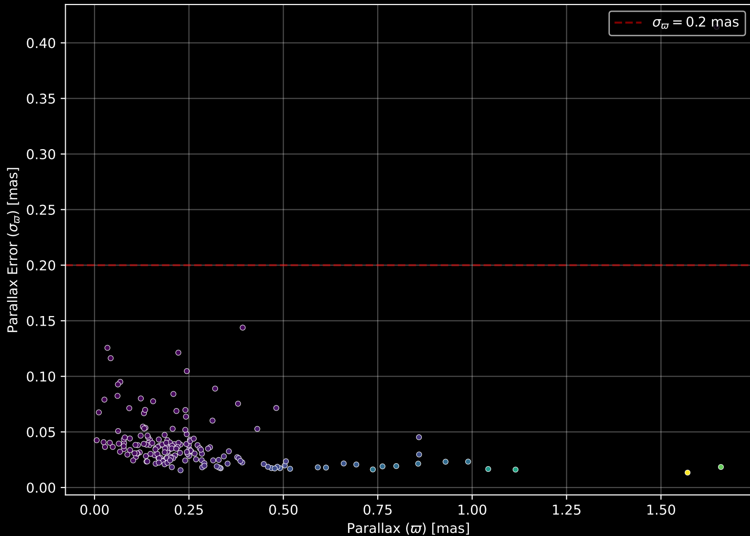
APOGEE DR17 Field: [024-03] Parallax Quality (n= 178)
