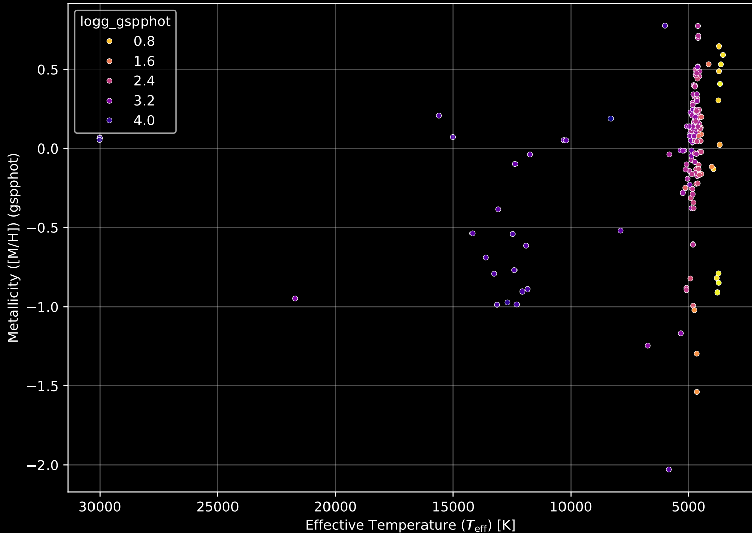
APOGEE DR17 Field: [024-03] Stellar Population Parameters (n= 178)
